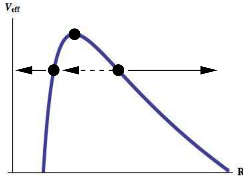
Figure 3. The effective potential eq. 4.15. There is a solution that sits precisely at the maximum, corresponding to AdS_2 \times S^2 . All other solutions correspond to some part of the RN spacetime; energies higher than the maximum of V_{\text{eff}} are super-extremal, equal to the maximum are extremal, and below the maximum are sub-extremal. The sub-extremal region between the horizons at r_+ and r_- corresponds to motion in an inverted potential between two turning points.
