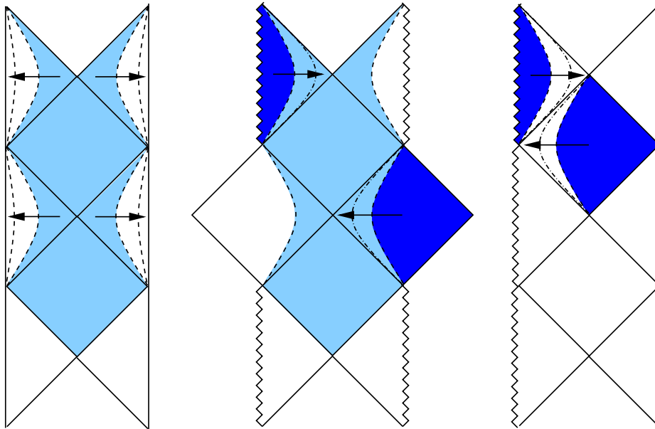
Figure 2. A pictorial representation of the limiting procedure. The AdS_2 \times S^2 space (left) and extremal black hole (right) can be obtained from different regions of the non-extremal black hole (center). For fixed constant r^* \sim \rho (dashed lines in the non-extremal black hole diagram), regions with smaller r (the light shaded portions of the diagram comprising Region II and portions of Regions I and III) are approximated close to extremality by the corresponding light shaded regions of the AdS_2 \times S^2 diagram. These interfaces approach the timelike boundaries of the AdS_2 \times S^2 space when extremality is approached ( \epsilon \rightarrow 0 ), as indicated by the arrows. The dark shaded regions on the non-extremal black hole diagram are approximated close to extremality by the corresponding dark shaded regions on the extremal black hole diagram. As extremality is approached, the extremal black hole approximation applies closer and closer to the horizon (as indicated by the arrows).
