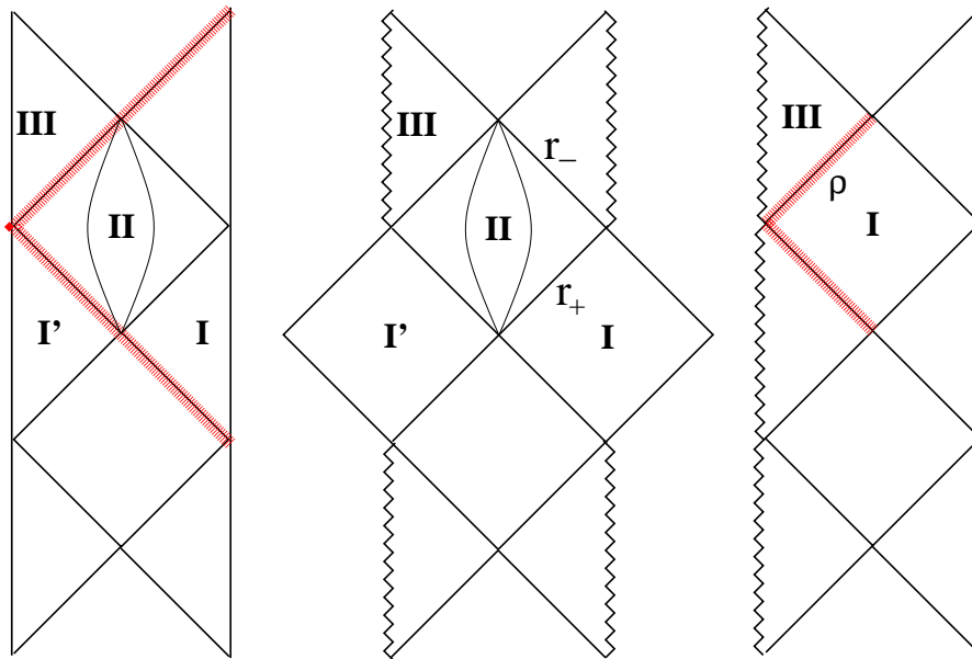
Figure 1. The causal structure of the AdS_2 space (left), non-extremal Reissner Nordström black hole (center), and the extremal Reissner Nordström black hole (right). The non-extremal black hole possesses two event horizons at r = r_+ and r = r_- , while the extremal black hole possesses only one at r = \rho . The solid lines in Region II of the non-extremal black hole are timelike trajectories of constant \psi (see eq. 3.2) extending from r_+ to r_- . The horizon of the extremal black hole solution indicated by the hatched red line is locally equivalent to the hatched red line of the AdS_2 diagram.
